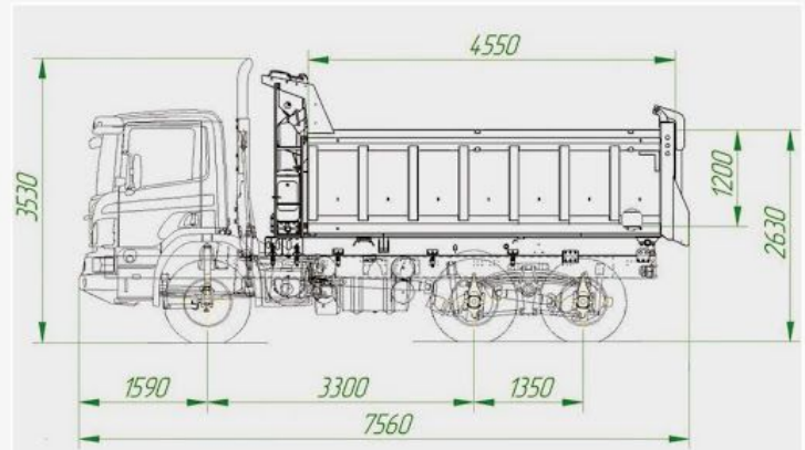
DC13 104 360 Euro 4
